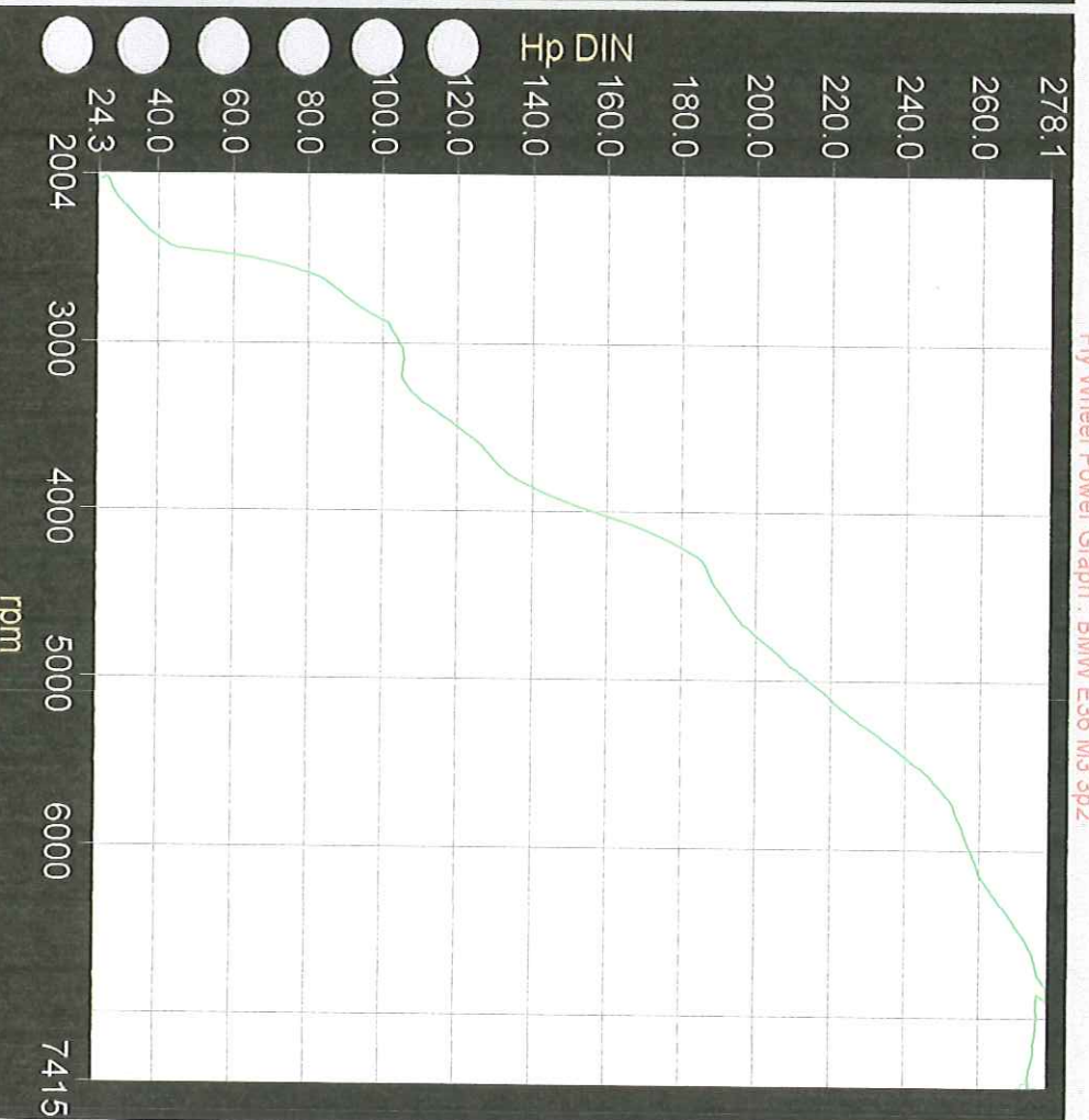
Fly Wheel Power Graph : BMW E36 M3 3p2
